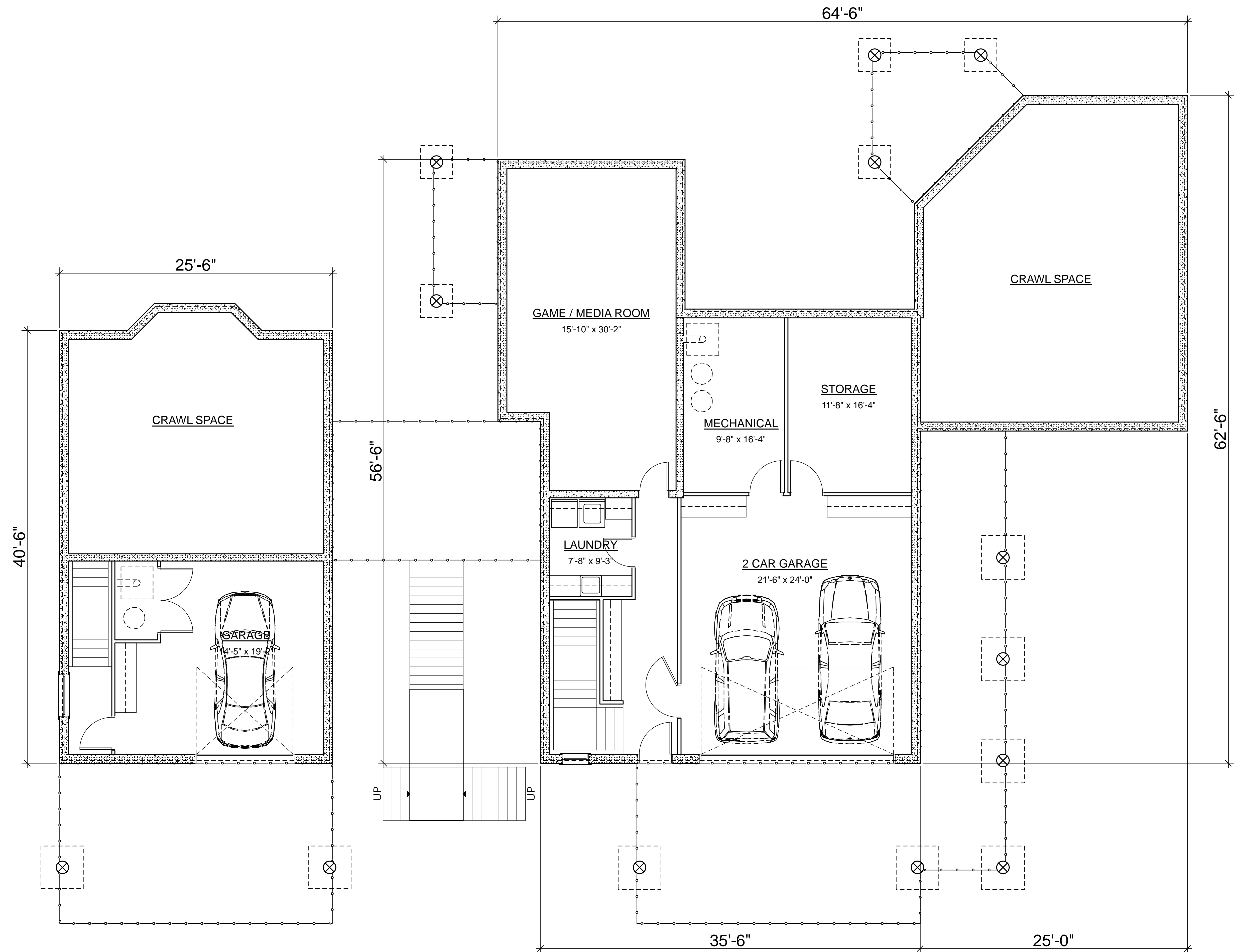
BASEMENT FLOOR PLAN AREA: MAIN HOUSE: 1, 200 SQ. FT. GARAGE 1: 560 SQ. FT., GARAGE 2: 380 SQ. FT.
